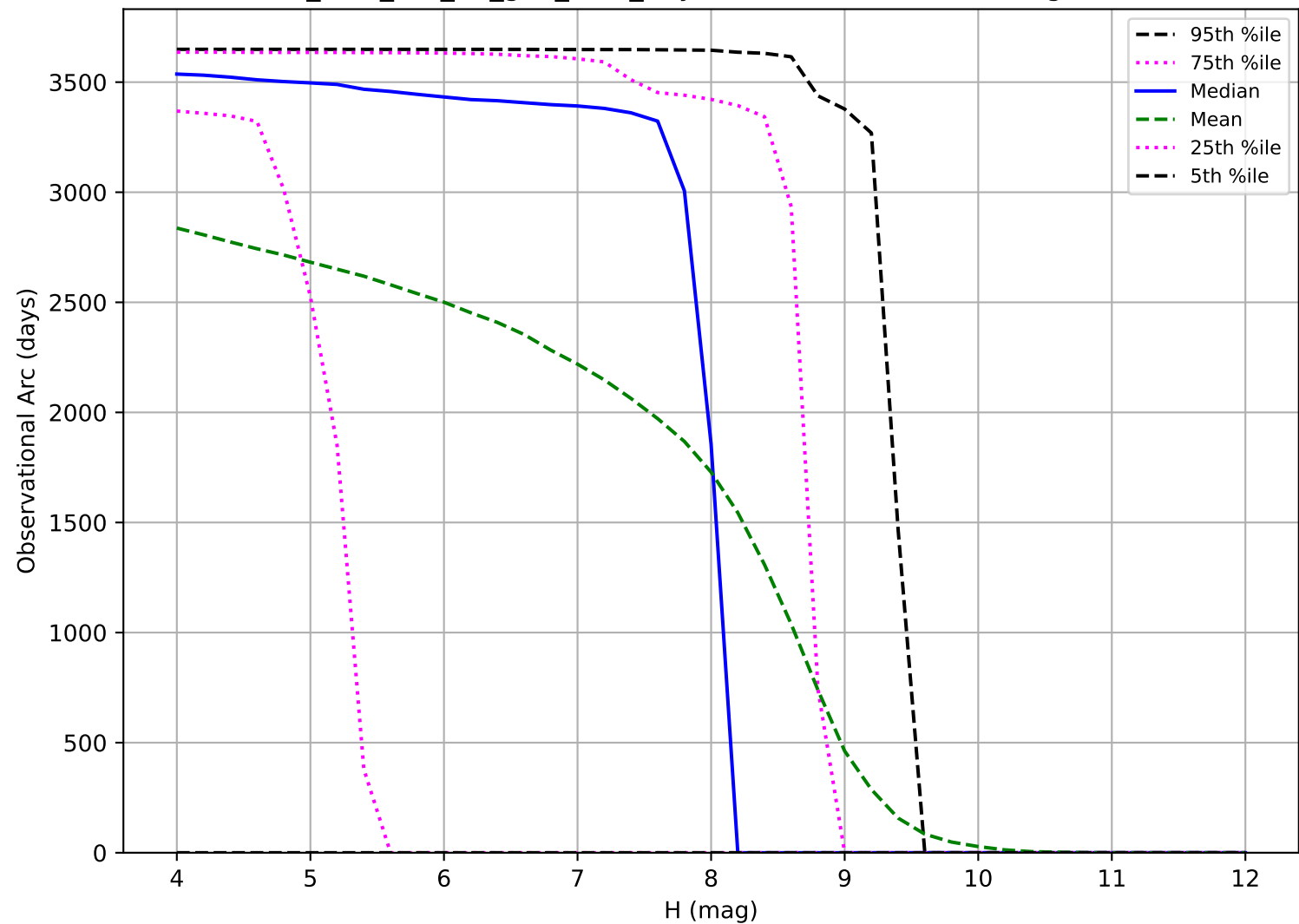
too_elab_r16_d3_griz_v3.4_10yrs: Observational Arc Length TNO
