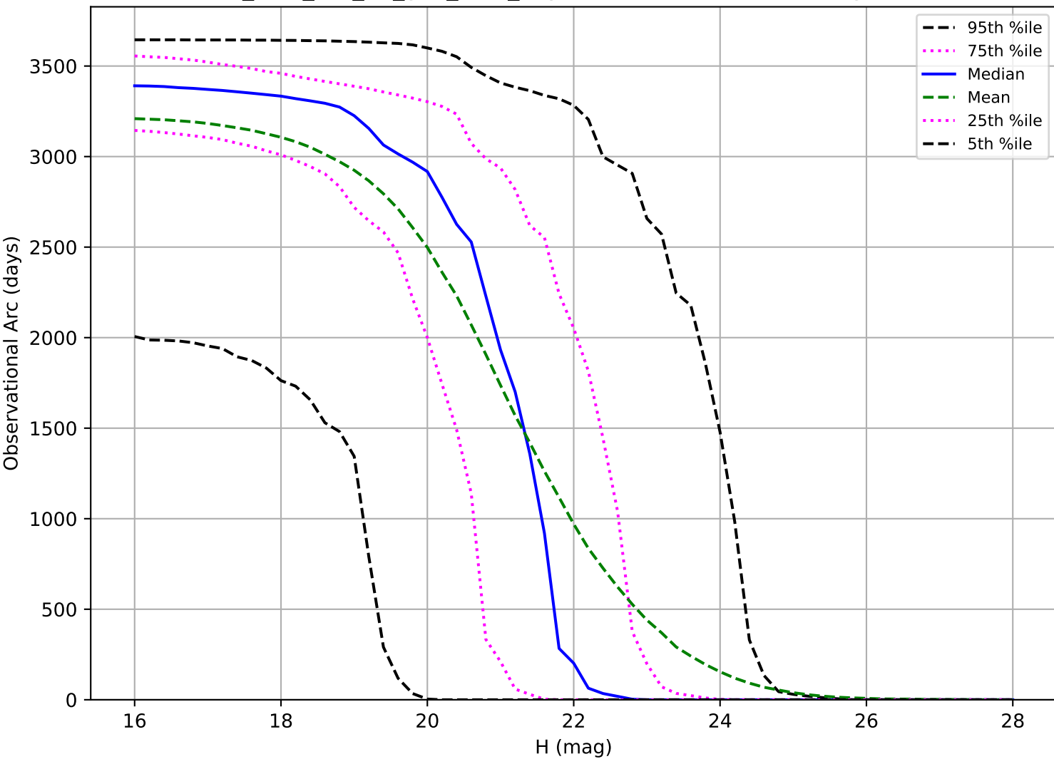
too_elab_r16_d3_griz_v3.4_10yrs: Observational Arc Length PHA
