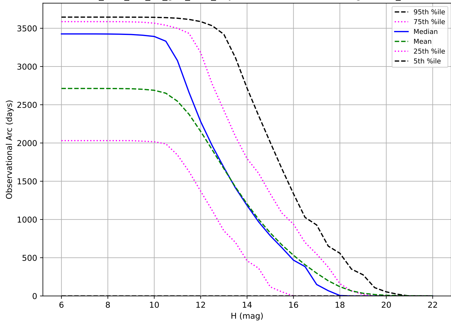
too_elab_r16_d3_griz_v3.4_10yrs: Observational Arc Length OCC_r5
