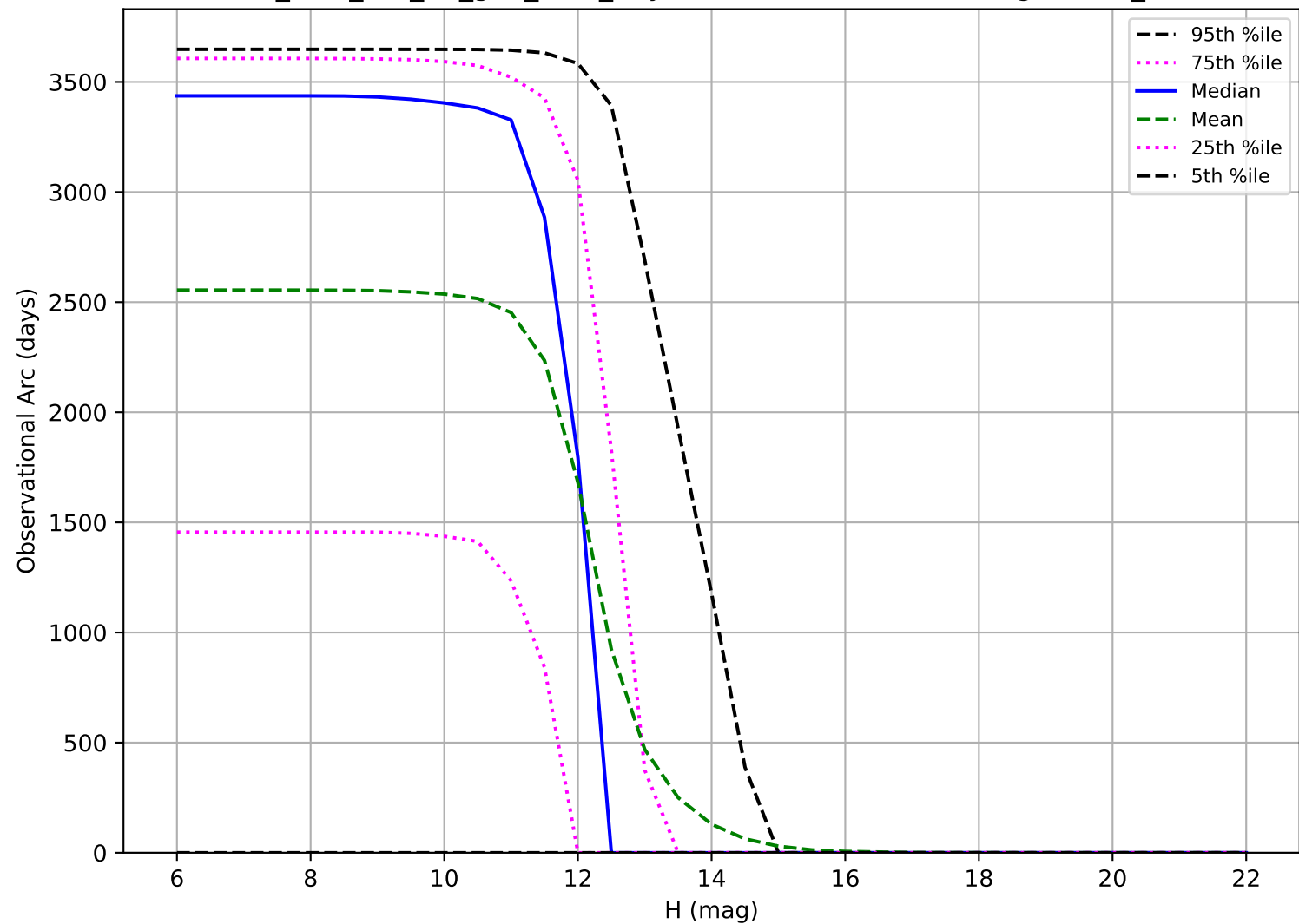
too_elab_r16_d3_griz_v3.4_10yrs: Observational Arc Length OCC_r20
