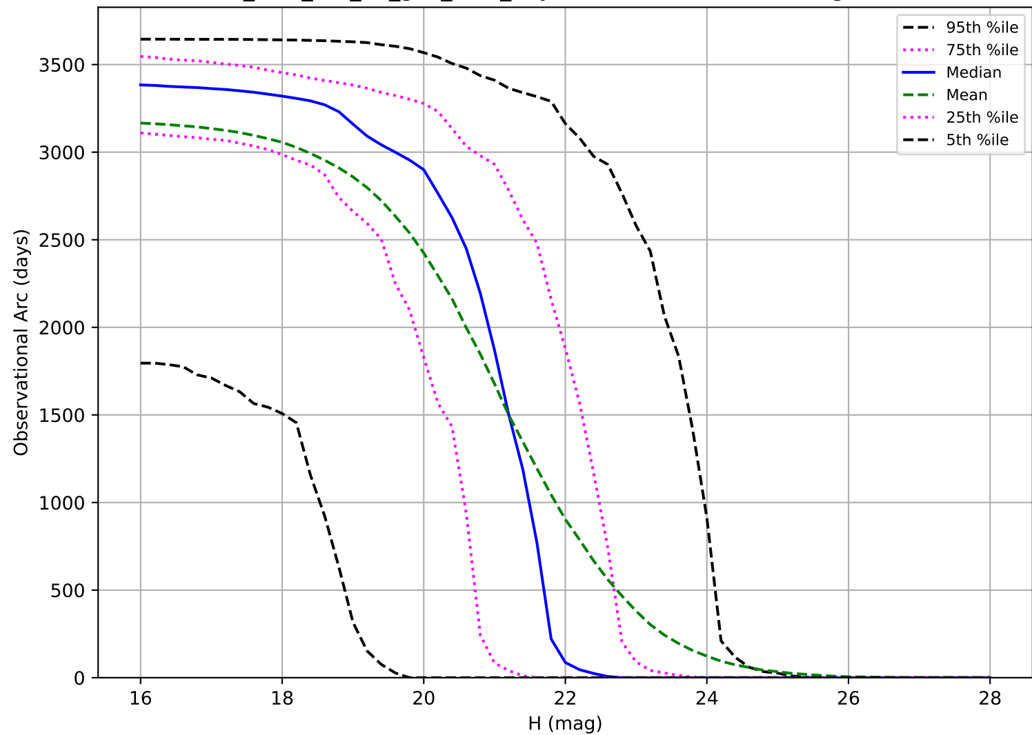
too_elab_r16_d3_griz_v3.4_10yrs: Observational Arc Length NEO
