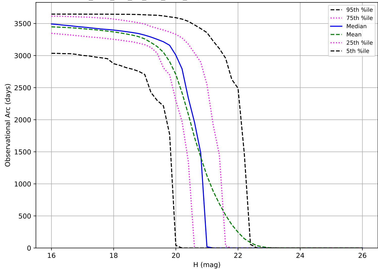
too_elab_r16_d3_griz_v3.4_10yrs: Observational Arc Length MBA
