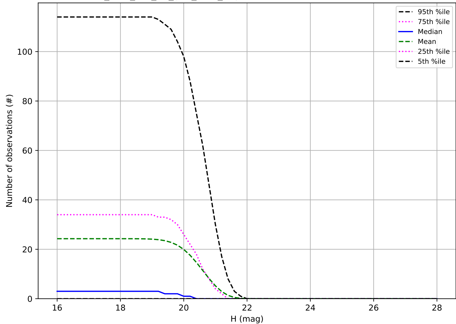
too_elab_r16_d3_griz_v3.4_10yrs: Number of observations Vatira
