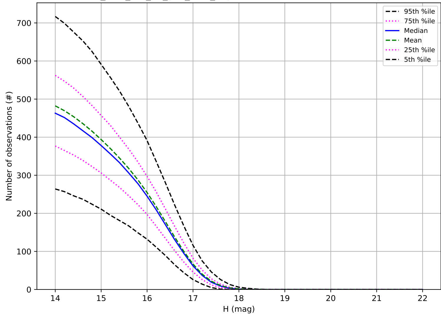
too_elab_r16_d3_griz_v3.4_10yrs: Number of observations Trojan
