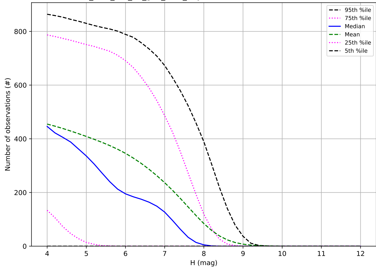
too_elab_r16_d3_griz_v3.4_10yrs: Number of observations TNO
