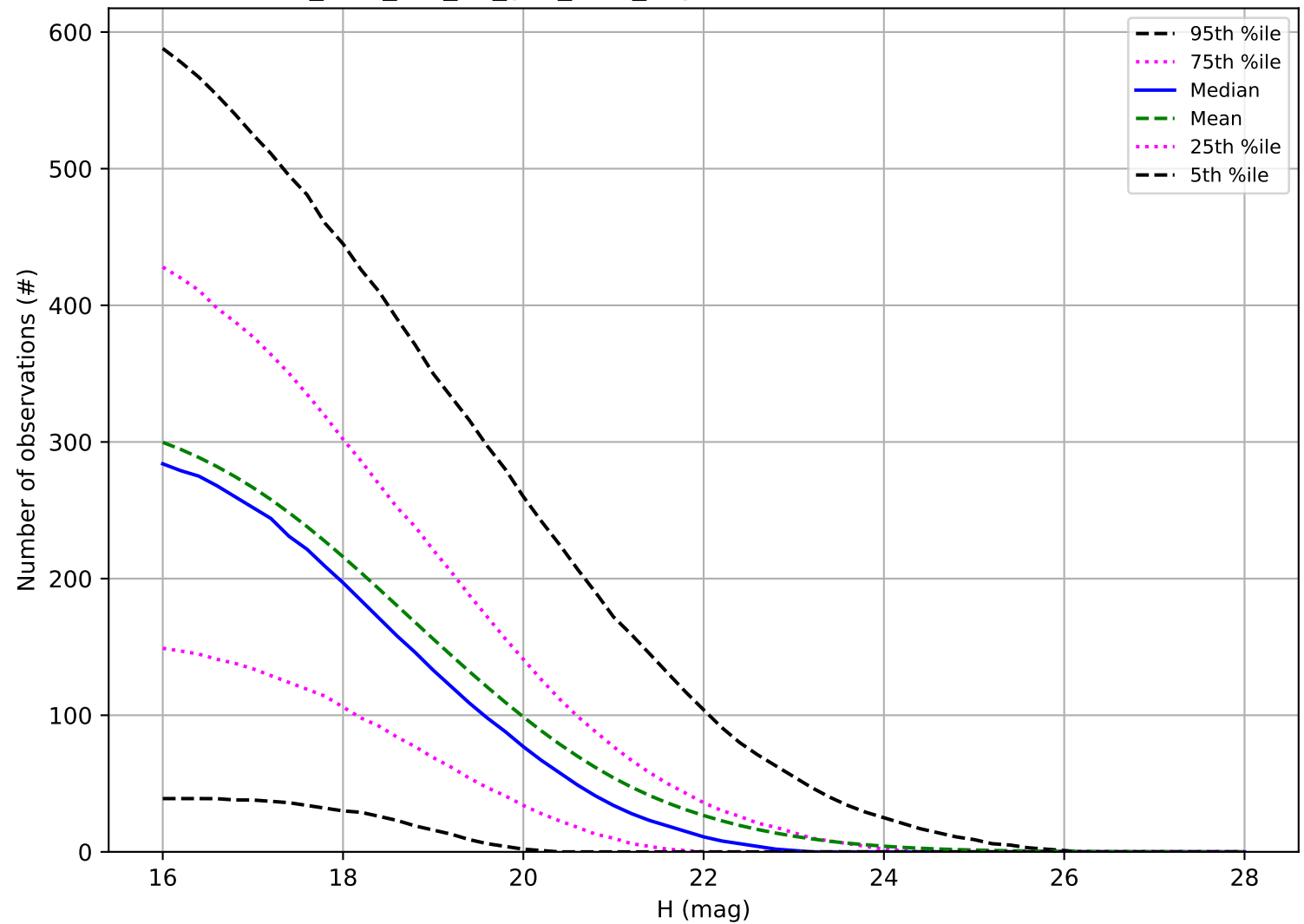
too_elab_r16_d3_griz_v3.4_10yrs: Number of observations PHA
