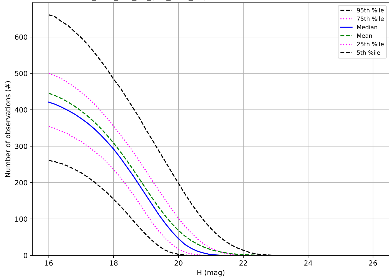
too_elab_r16_d3_griz_v3.4_10yrs: Number of observations MBA
