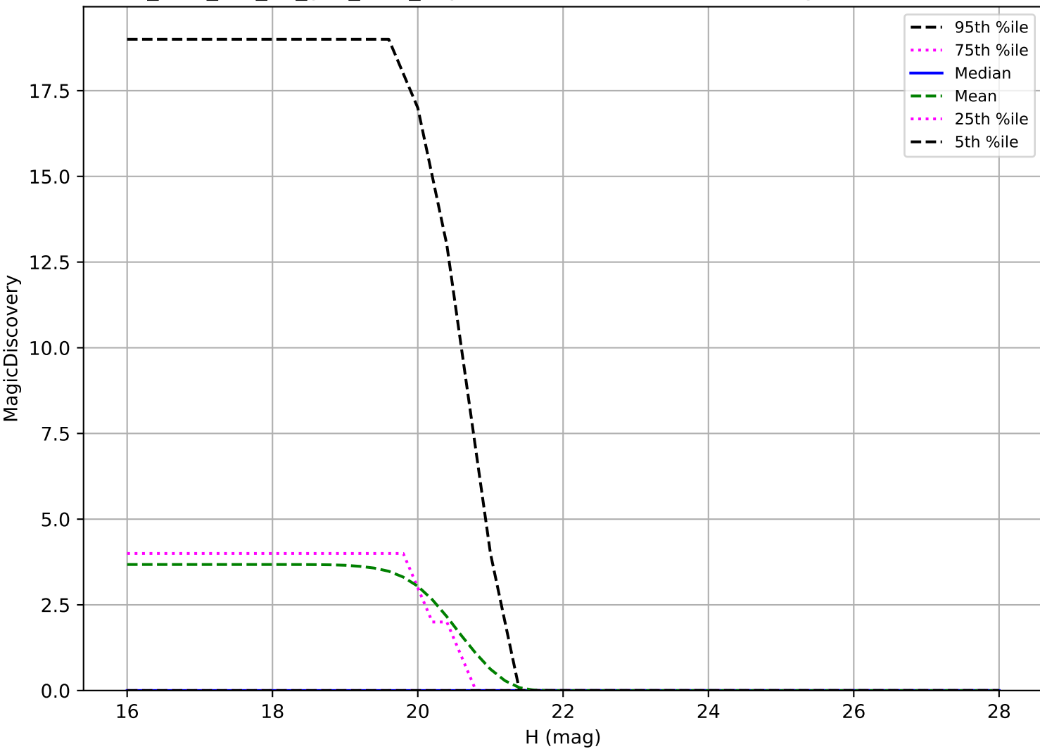
too_elab_r16_d3_griz_v3.4_10yrs: Vatira 6 detections in 60 nights detection loss
