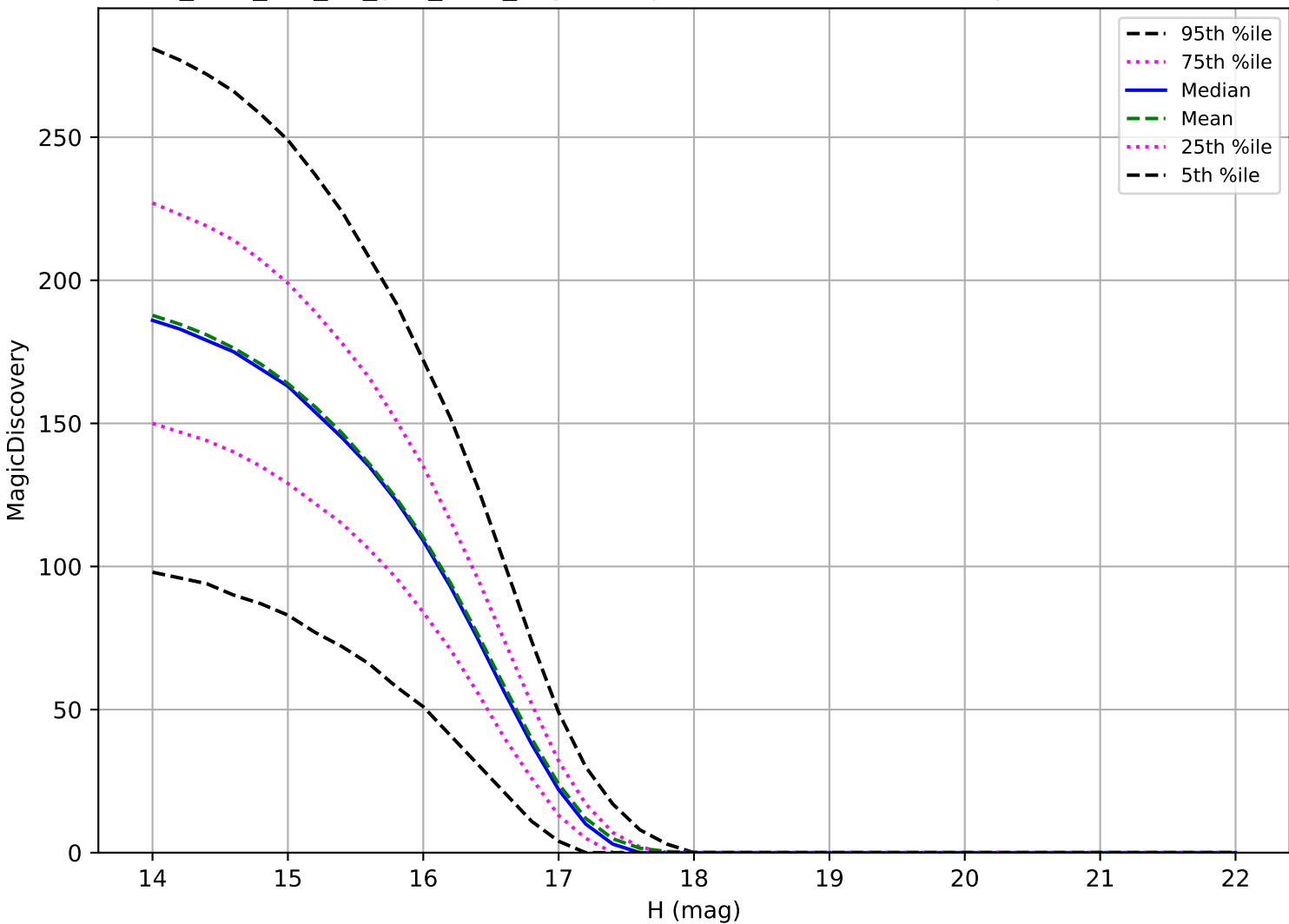
too_elab_r16_d3_griz_v3.4_10yrs: Trojan 6 detections in 60 nights detection loss
