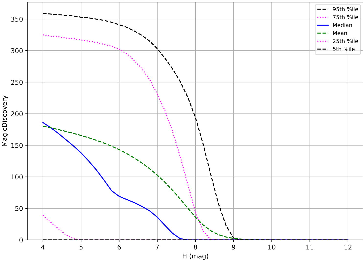
too_elab_r16_d3_griz_v3.4_10yrs: TNO 6 detections in 60 nights detection loss
