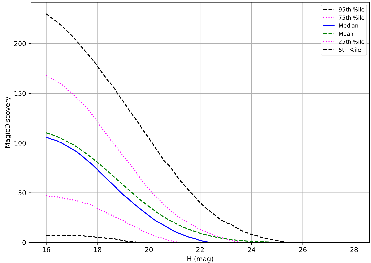
too_elab_r16_d3_griz_v3.4_10yrs: PHA 6 detections in 60 nights detection loss
