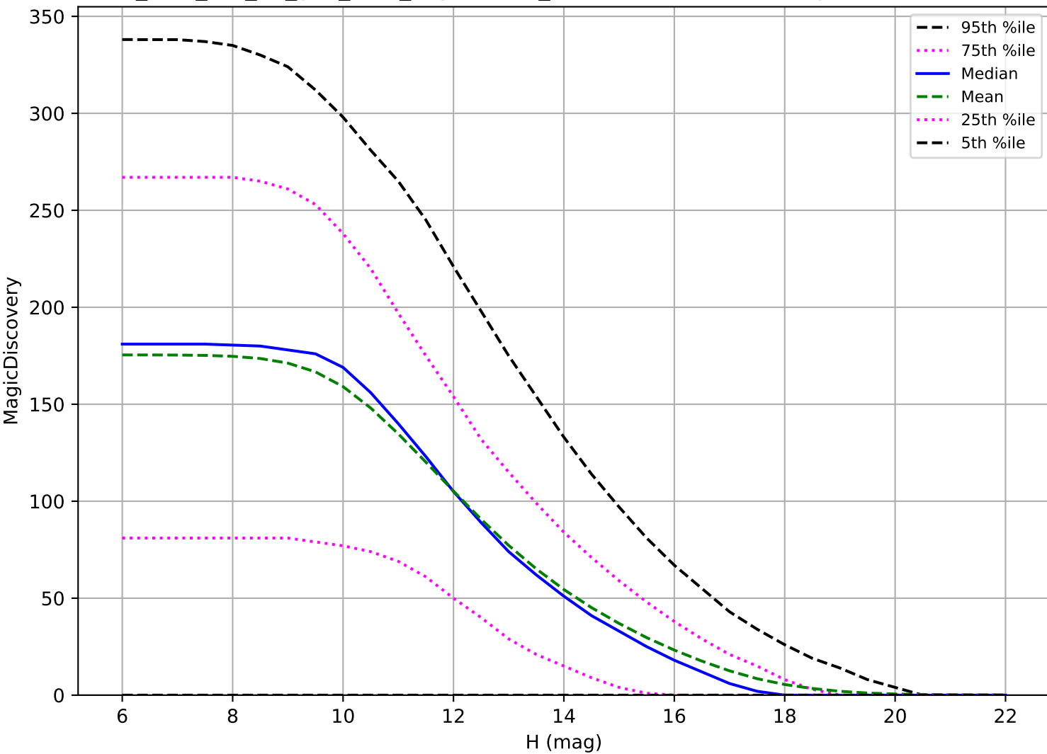
too_elab_r16_d3_griz_v3.4_10yrs: OCC_r5 6 detections in 60 nights detection loss
