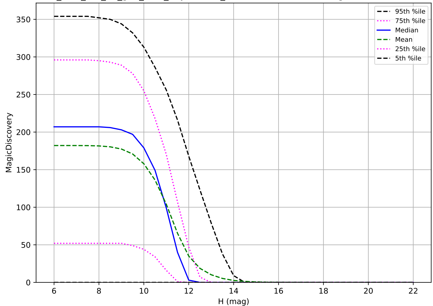
too_elab_r16_d3_griz_v3.4_10yrs: OCC_r20 6 detections in 60 nights detection loss
