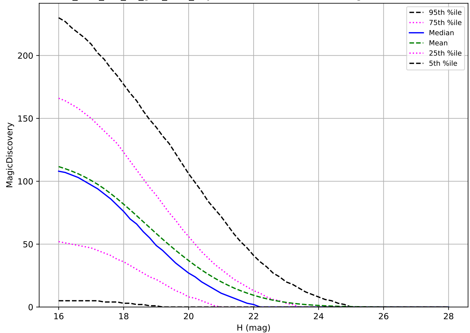
too_elab_r16_d3_griz_v3.4_10yrs: NEO 6 detections in 60 nights detection loss
