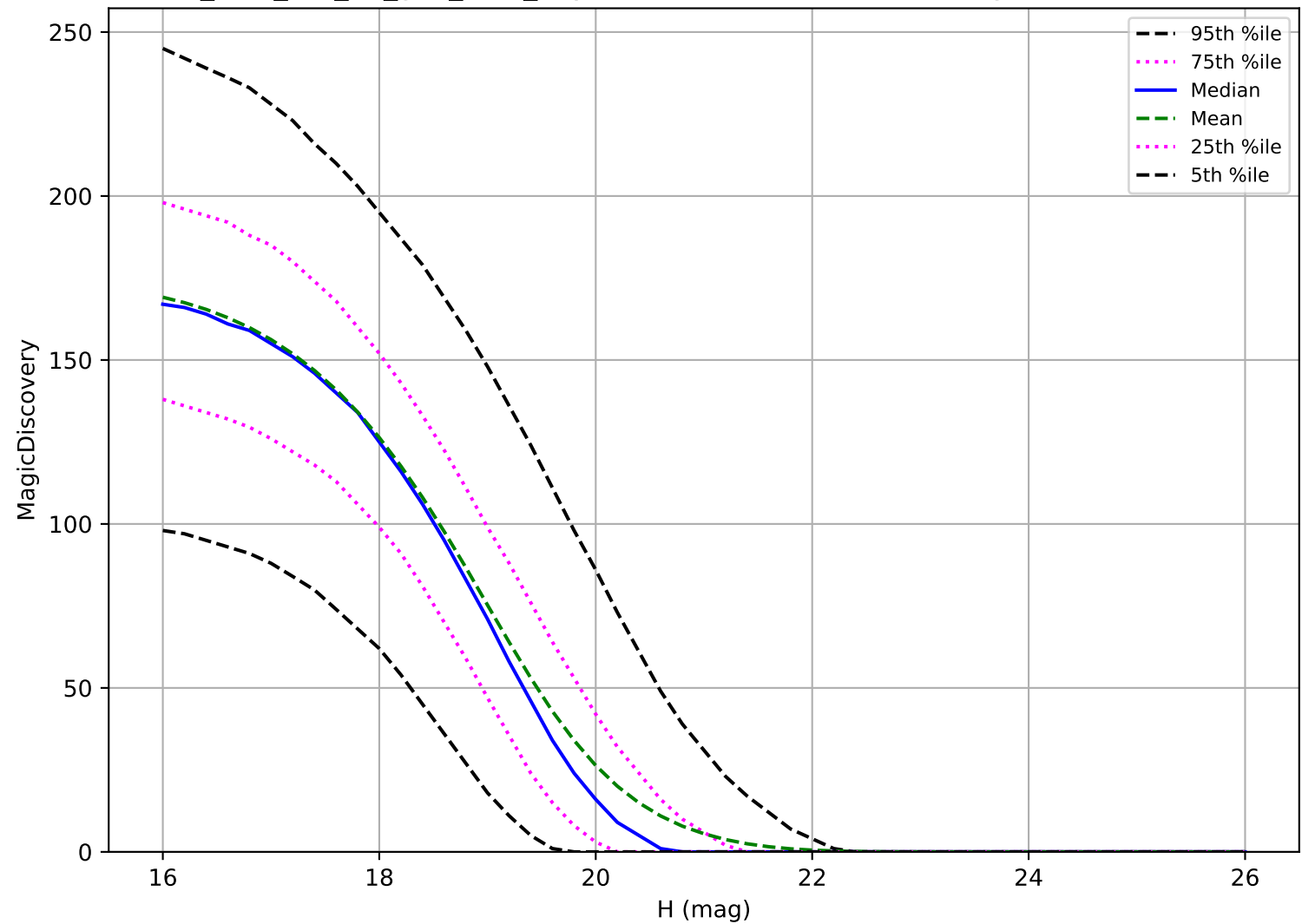
too_elab_r16_d3_griz_v3.4_10yrs: MBA 6 detections in 60 nights detection loss
