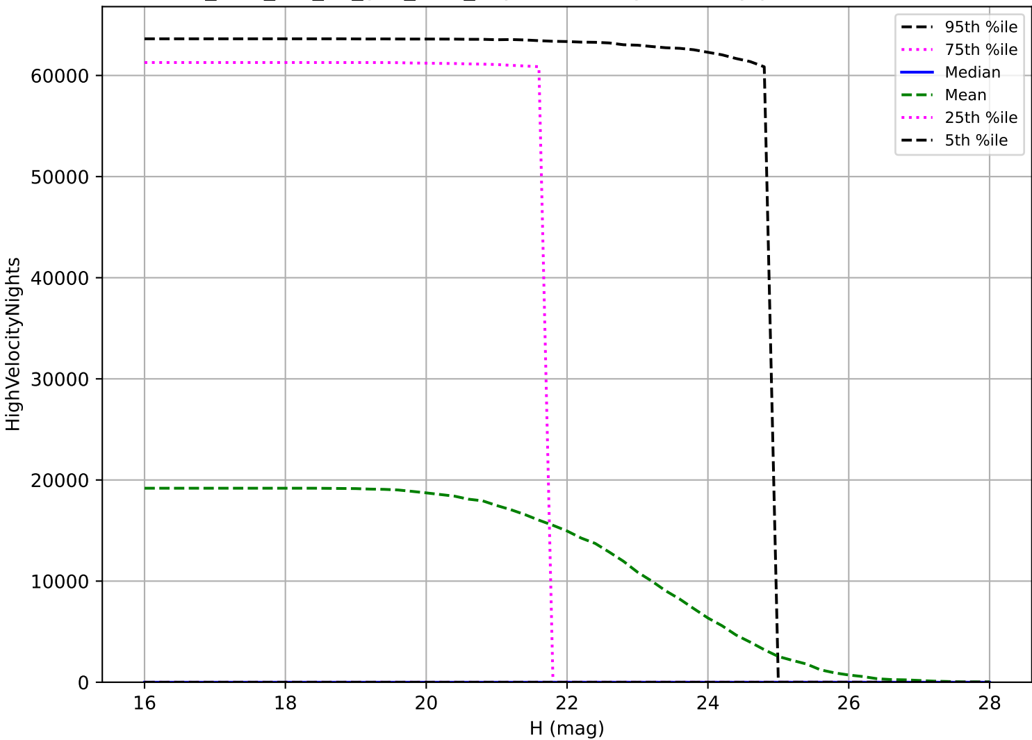
too_elab_r16_d3_griz_v3.4_10yrs: NEO High velocity pair detection loss
