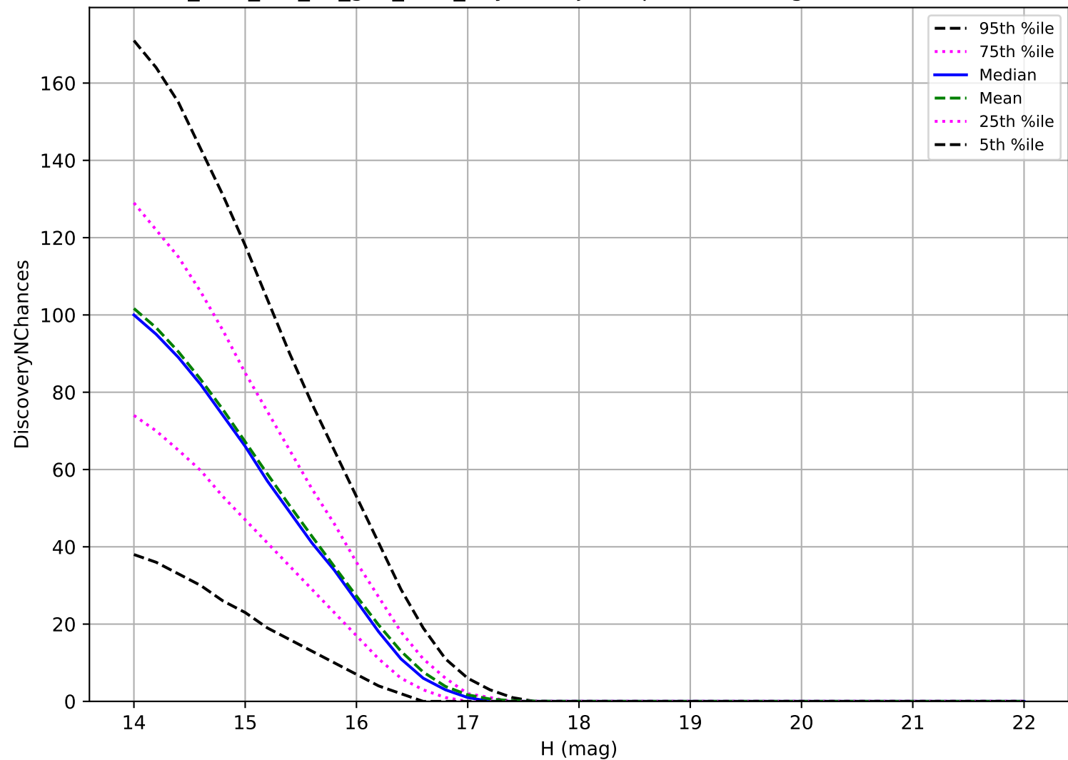
too_elab_r16_d3_griz_v3.4_10yrs: Trojan 3 pairs in 15 nights detection loss
