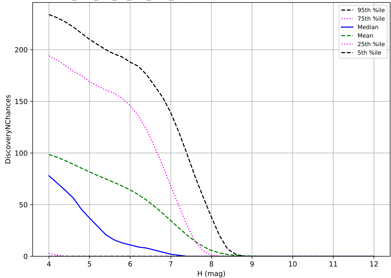
too_elab_r16_d3_griz_v3.4_10yrs: TNO 3 pairs in 15 nights detection loss
