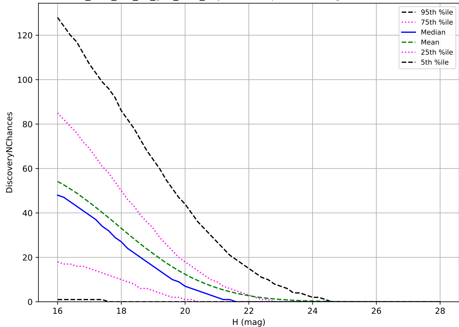
too_elab_r16_d3_griz_v3.4_10yrs: PHA 3 pairs in 15 nights detection loss
