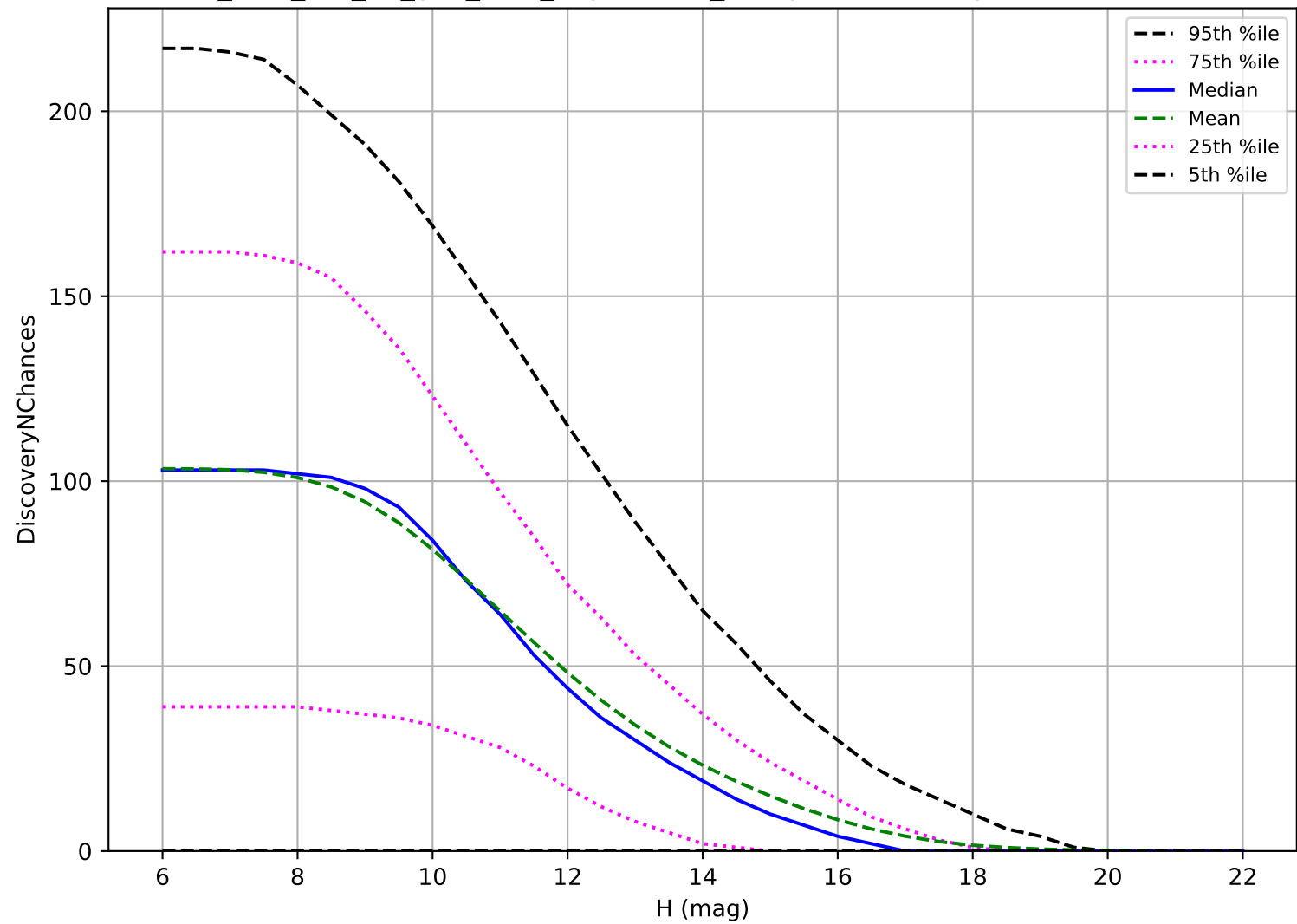
too_elab_r16_d3_griz_v3.4_10yrs: OCC_r5 3 pairs in 15 nights detection loss
