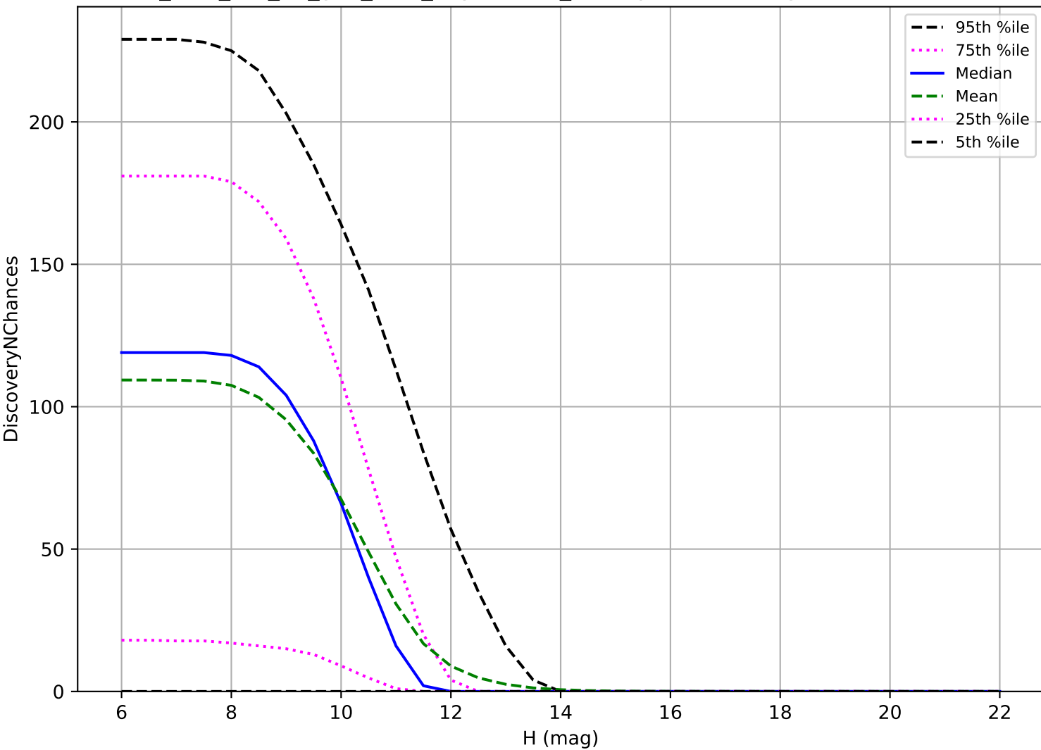
too_elab_r16_d3_griz_v3.4_10yrs: OCC_r20 3 pairs in 15 nights detection loss
