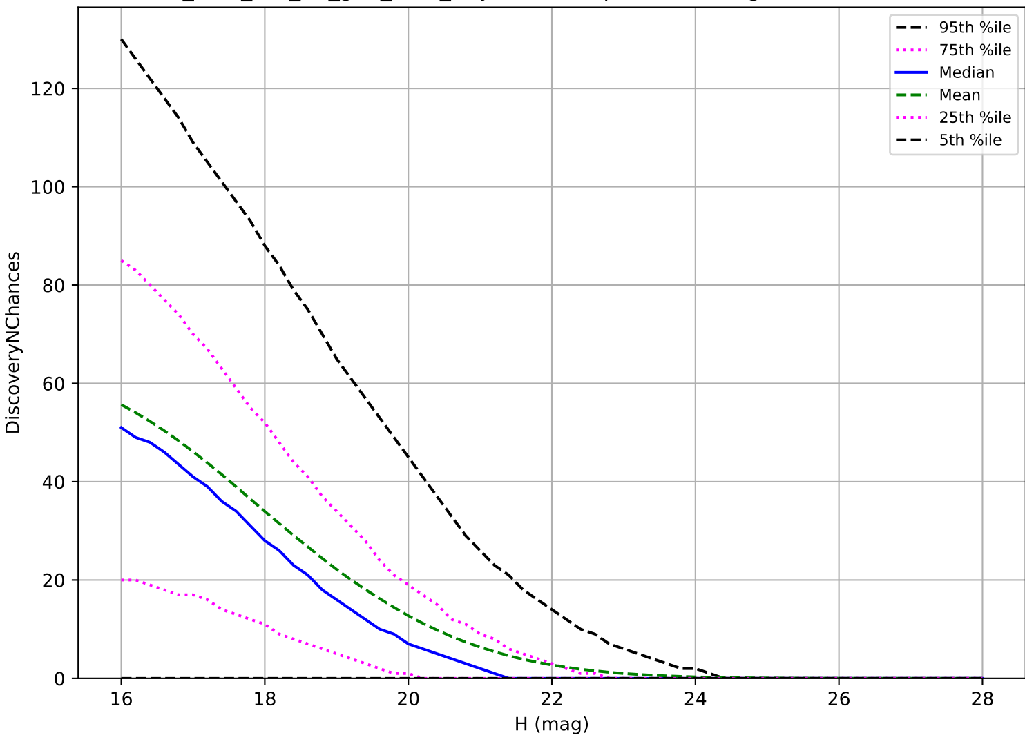
too_elab_r16_d3_griz_v3.4_10yrs: NEO 3 pairs in 15 nights detection loss
