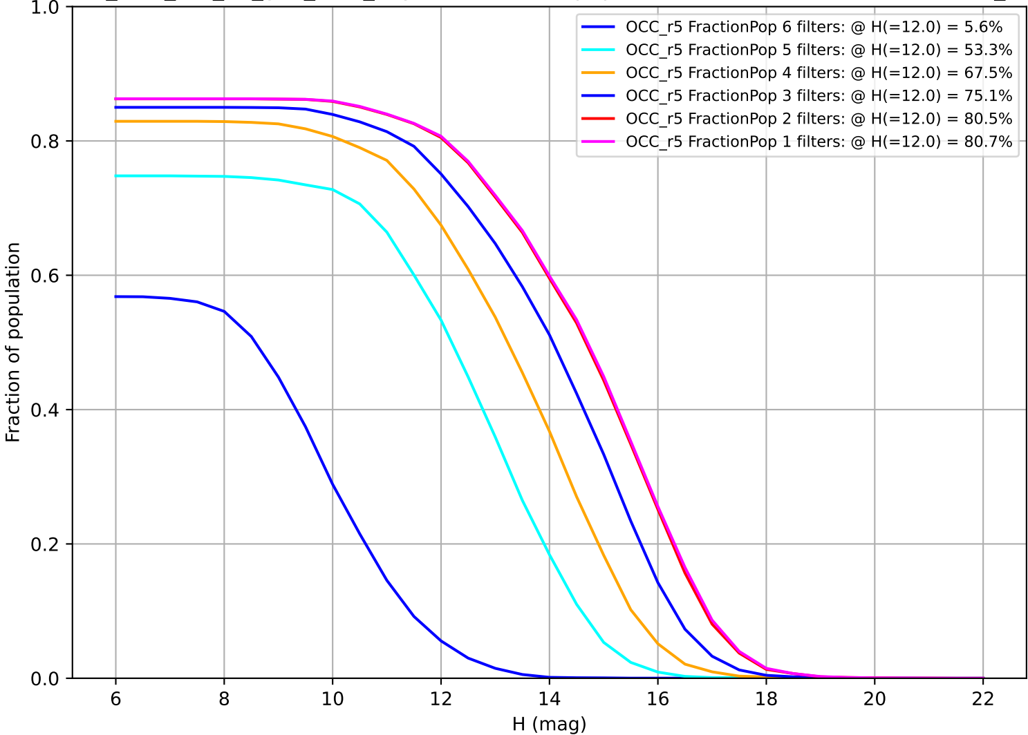
too_elab_r16_d3_griz_v3.4_10yrs: Fraction of population with colors in X filters OCC_r5
