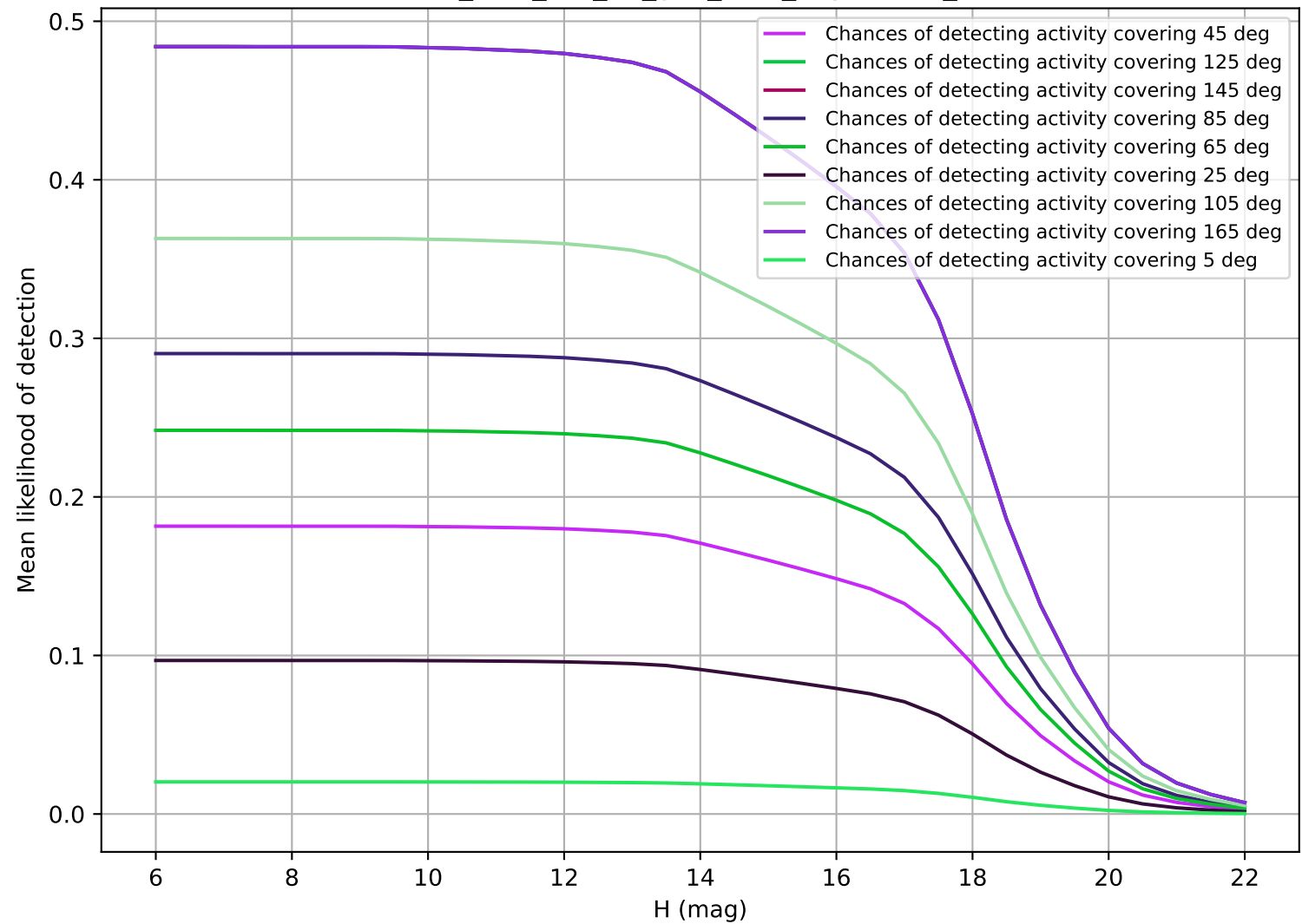
too_elab_r16_d3_griz_v3.4_10yrs OCC_r5
