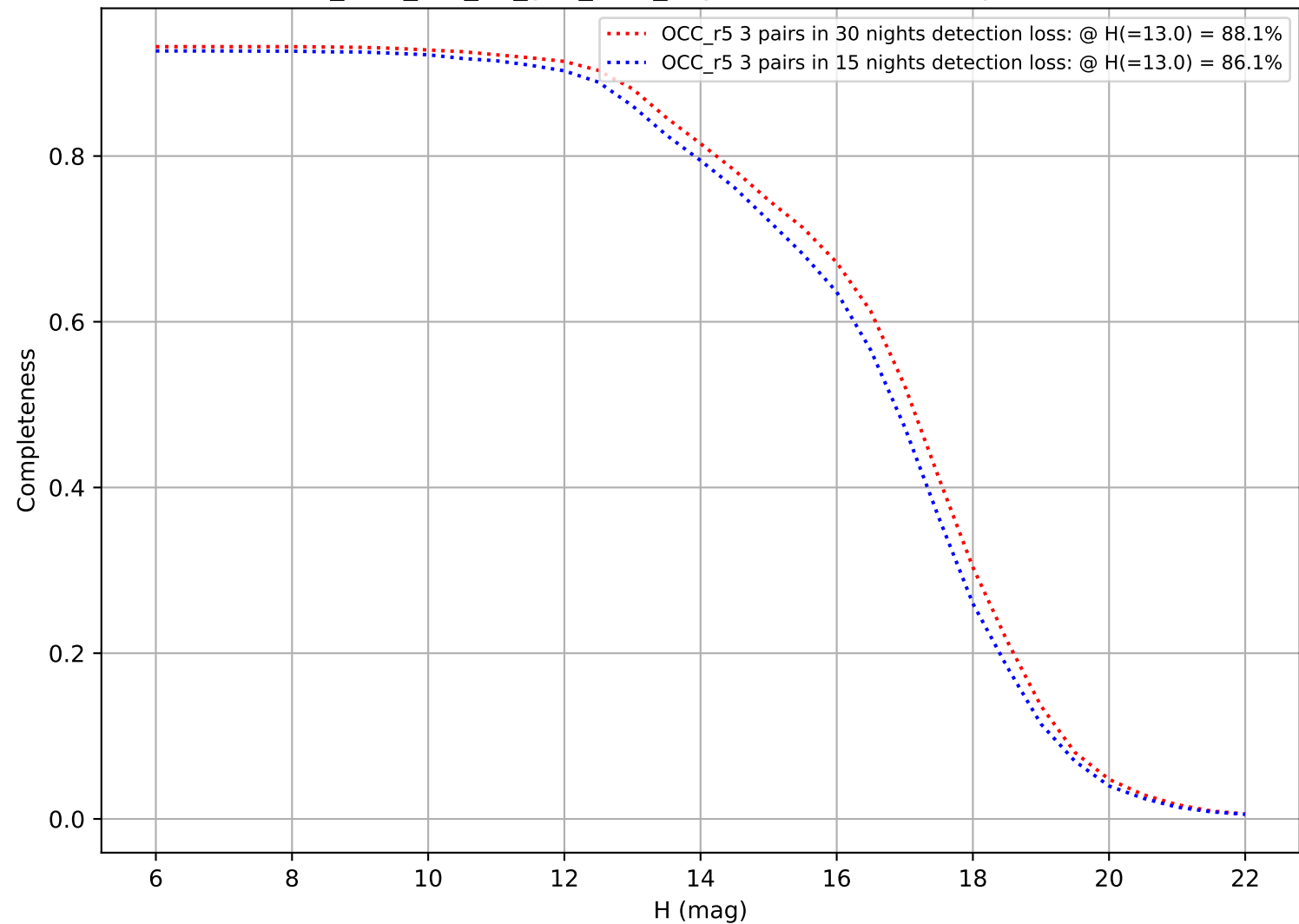
too_elab_r16_d3_griz_v3.4_10yrs: DifferentialCompleteness
