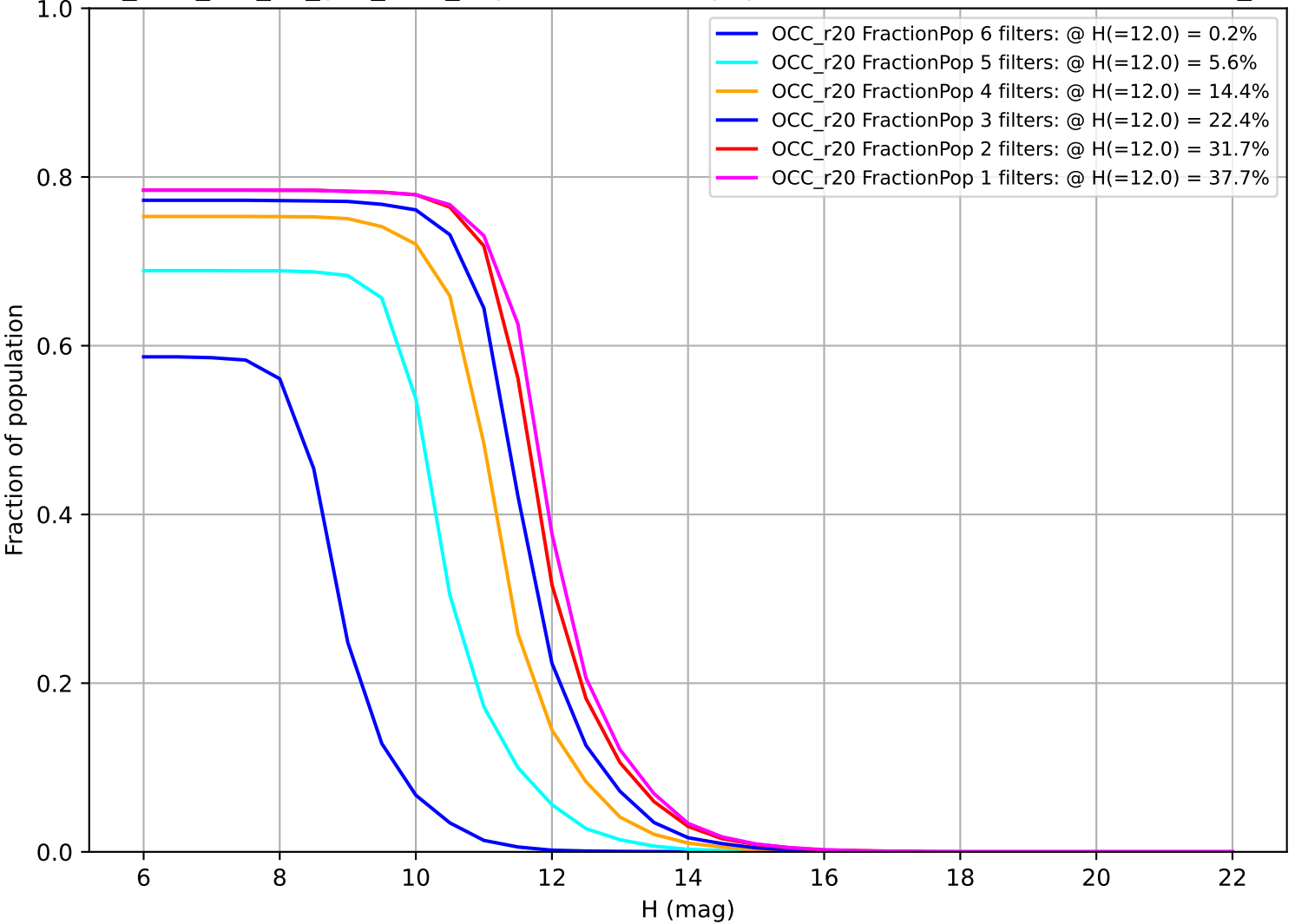
too_elab_r16_d3_griz_v3.4_10yrs: Fraction of population with colors in X filters OCC_r20
