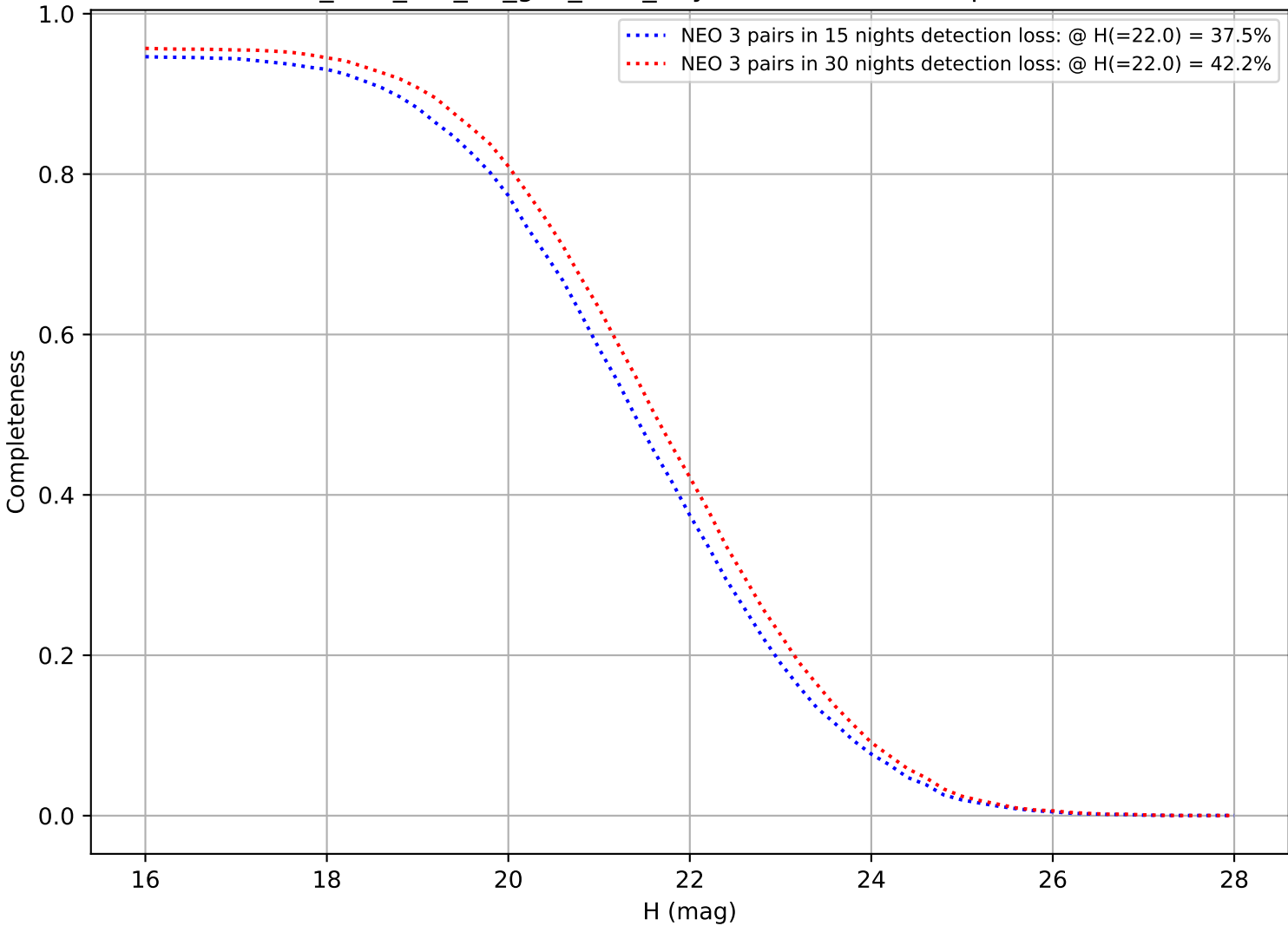
too_elab_r16_d3_griz_v3.4_10yrs: DifferentialCompleteness
