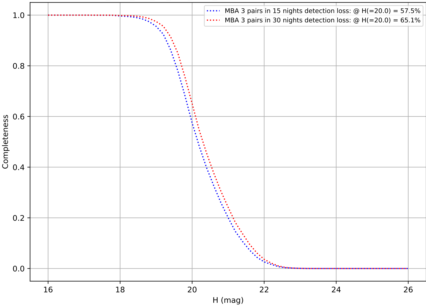
too_elab_r16_d3_griz_v3.4_10yrs: DifferentialCompleteness
