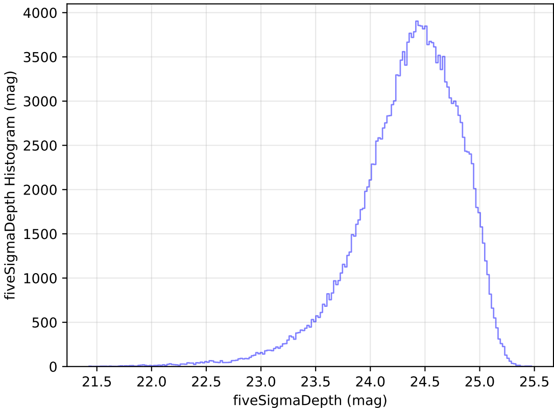
too_elab_r16_d3_griz_v3.4_10yrs g: fiveSigmaDepth Histogram
