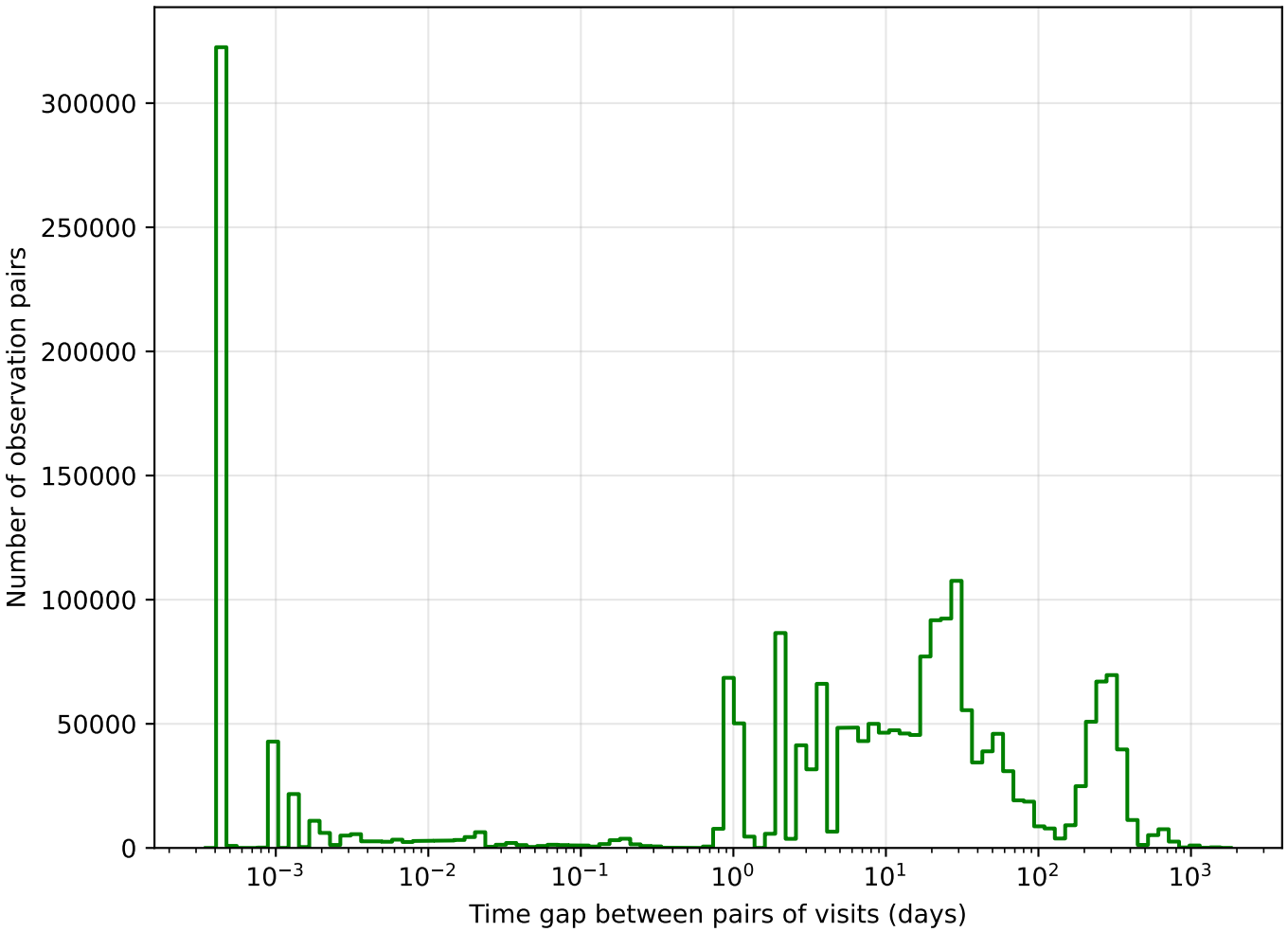
too_elab_r16_d3_griz_v3.4_10yrs g band: Tgaps observationStartMJD
