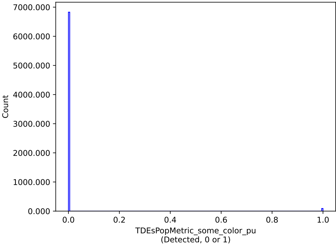
too_elab_r16_d3_griz_v3.4_10yrs : TDEsPopMetric_some_color_pu
