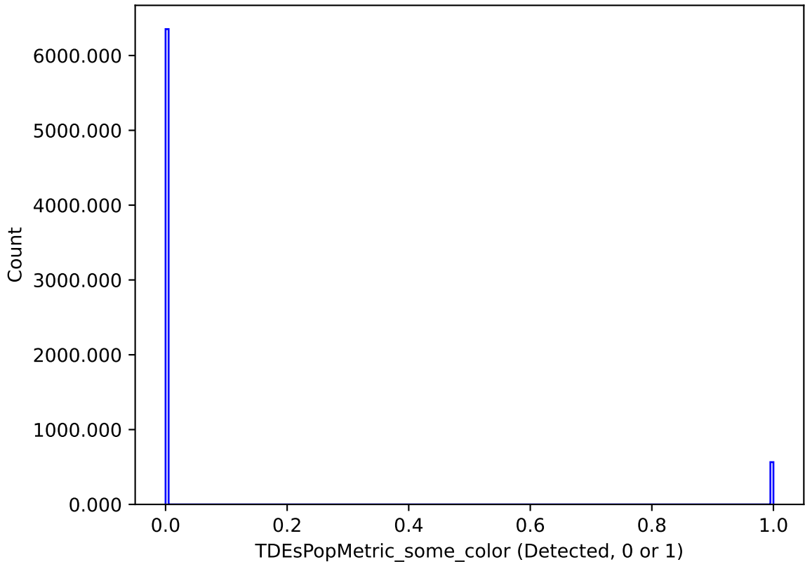
too_elab_r16_d3_griz_v3.4_10yrs : TDEsPopMetric_some_color
