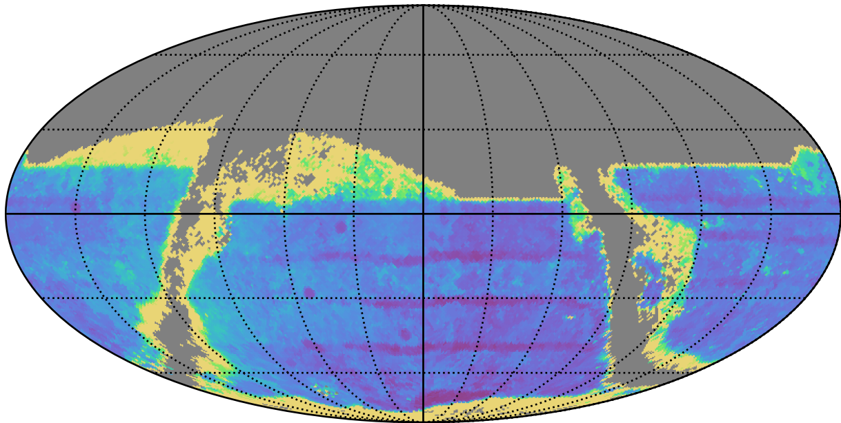
too_elab_r16_d3_griz_v3.4_10yrs : TDC_accuracy
