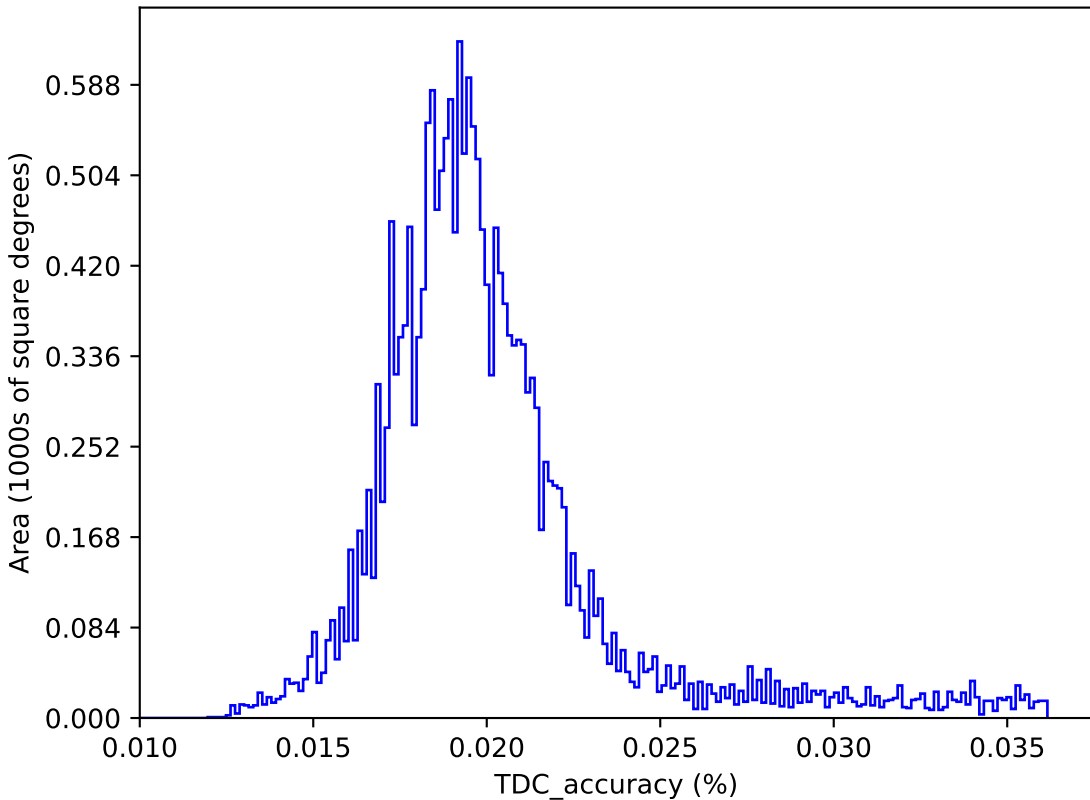
too_elab_r16_d3_griz_v3.4_10yrs : TDC_accuracy
