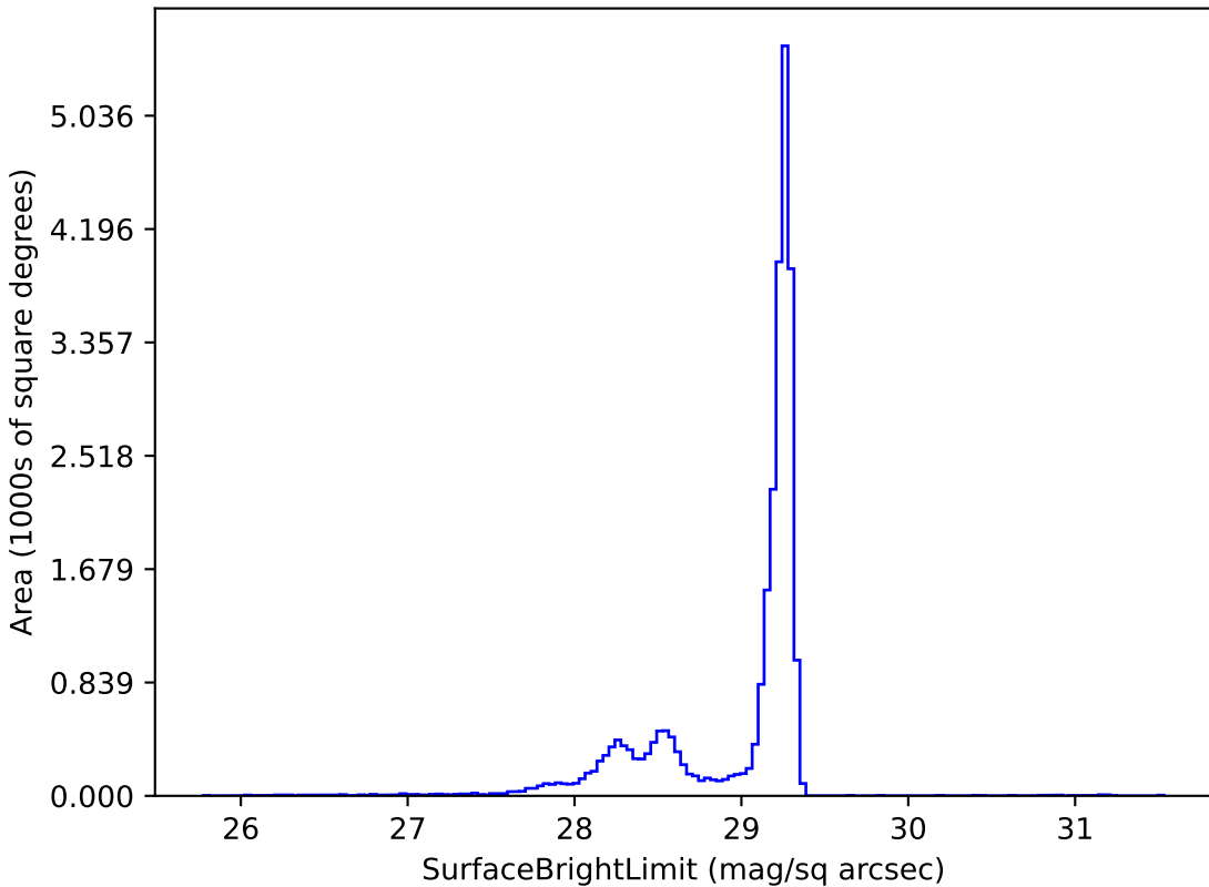
too_elab_r16_d3_griz_v3.4_10yrs z: SurfaceBrightLimit
