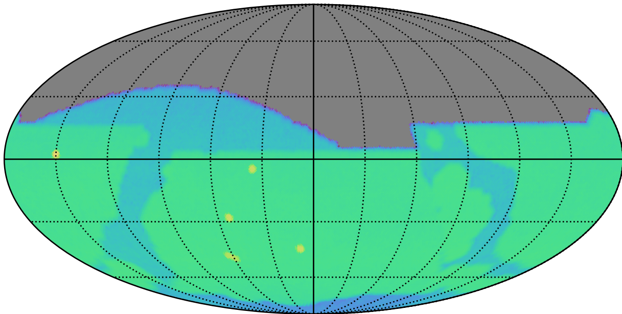
too_elab_r16_d3_griz_v3.4_10yrs r: SurfaceBrightLimit
