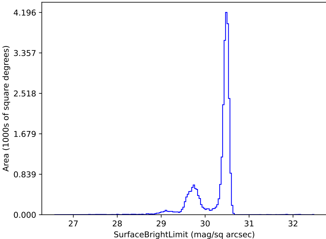
too_elab_r16_d3_griz_v3.4_10yrs r: SurfaceBrightLimit
