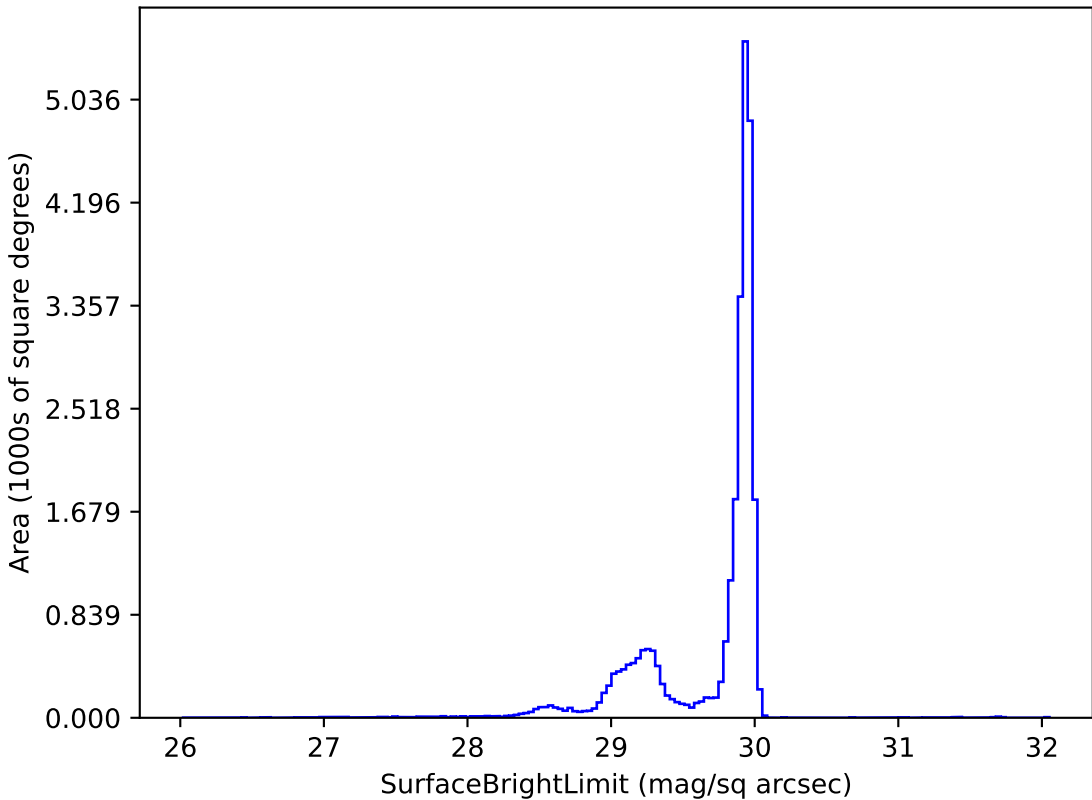
too_elab_r16_d3_griz_v3.4_10yrs i: SurfaceBrightLimit
