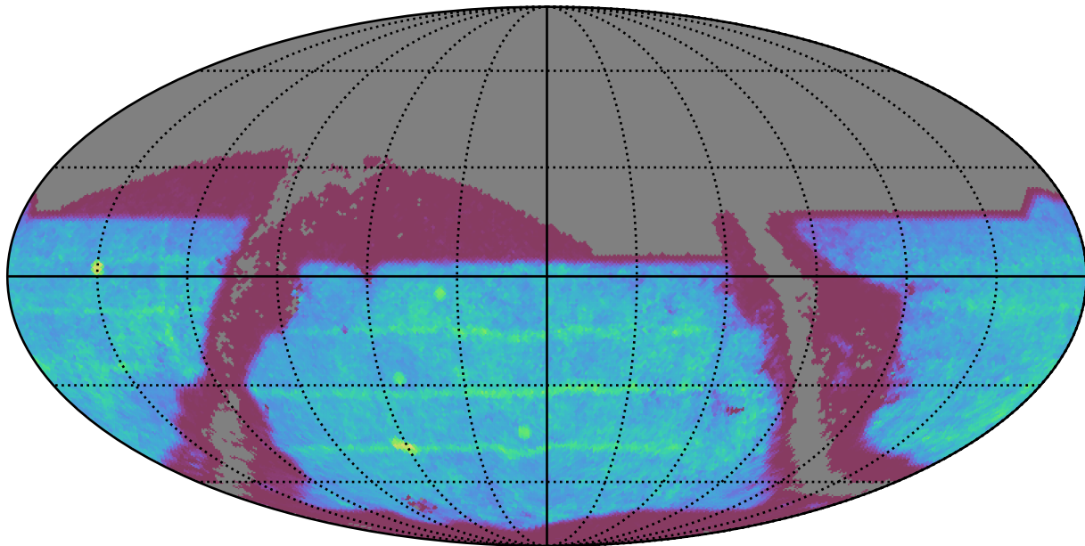
too_elab_r16_d3_griz_v3.4_10yrs : SNSLMetric
