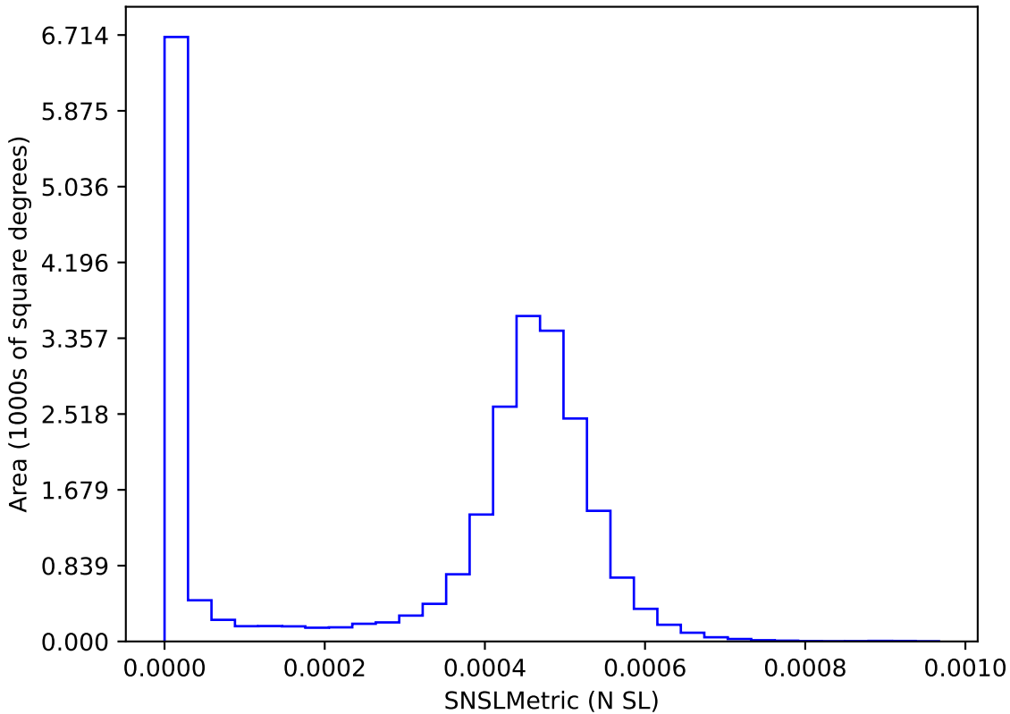
too_elab_r16_d3_griz_v3.4_10yrs : SNSLMetric
