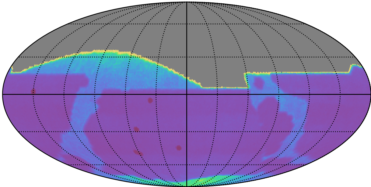
too_elab_r16_d3_griz_v3.4_10yrs : Proper Motion Uncert @ 20.5
