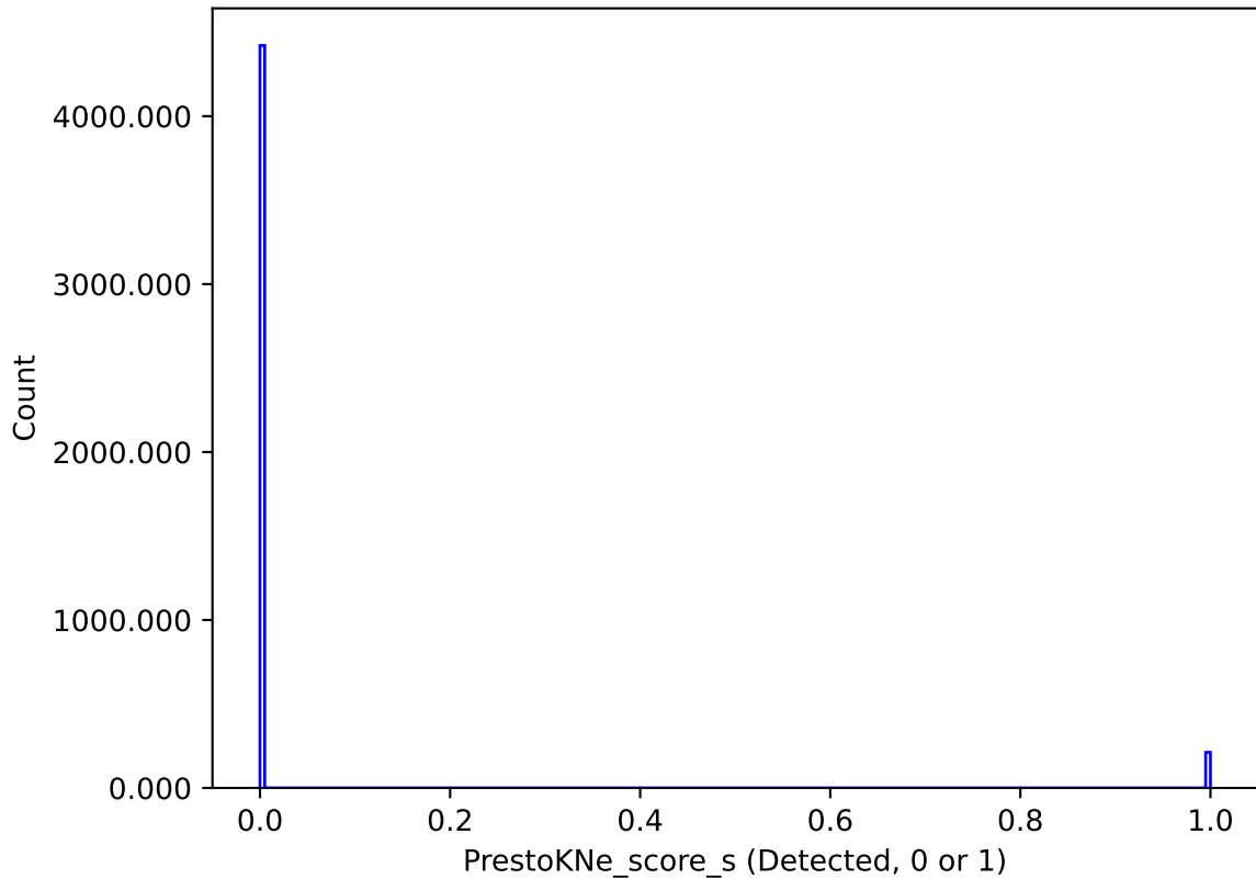
too_elab_r16_d3_griz_v3.4_10yrs : PrestoKNe_score_s
