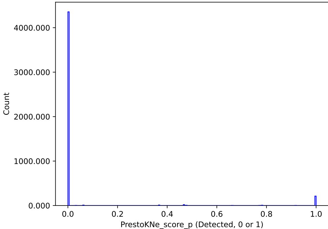
too_elab_r16_d3_griz_v3.4_10yrs : PrestoKNe_score_p
