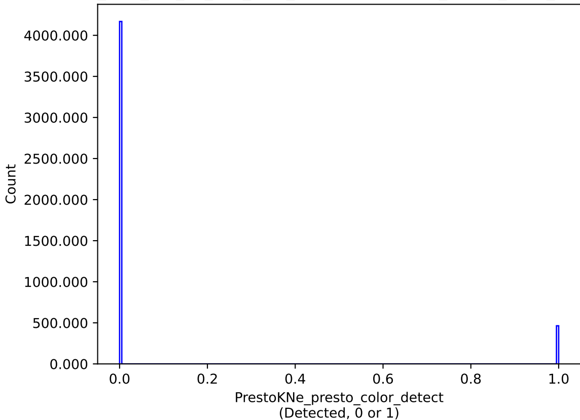
too_elab_r16_d3_griz_v3.4_10yrs : PrestoKNe_presto_color_detect
