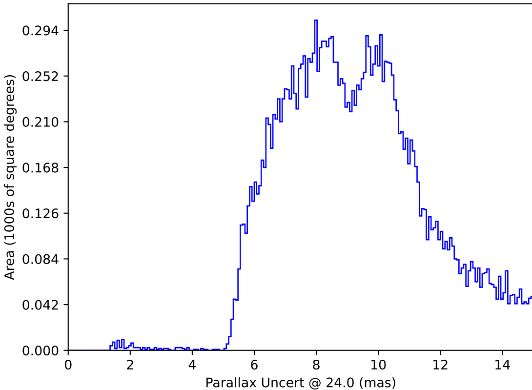
too_elab_r16_d3_griz_v3.4_10yrs : Parallax Uncert @ 24.0
