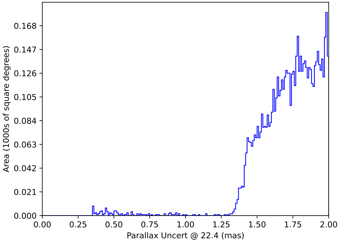
too_elab_r16_d3_griz_v3.4_10yrs : Parallax Uncert @ 22.4
